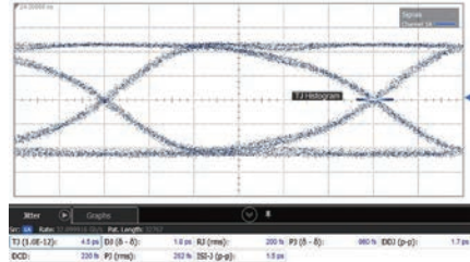
28 Gbit/s, PPG Intrinsic TJ (1E-12) = 4.5 psp-p, RJ rms = 200 fs Nominal measured data.
